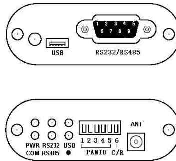
PC2ZB-Dimension figure
