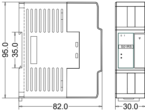
S01RS, H01ZB-Dimension figure
